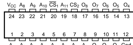
24 Lead Ceramic DIP/24 Lead Leaded Chip Carrier/24 Lead Sidebraced
